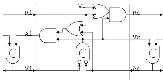
Figure 13: Correct anti-token latch design
