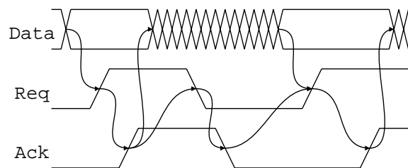
Figure 1: Four phase protocol
