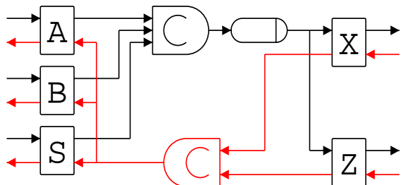
Figure 5: Naive circuit control
