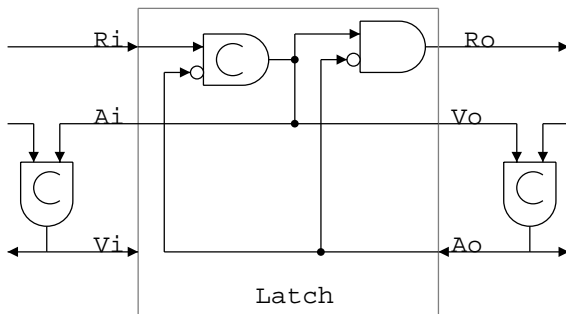
Figure 11: Early output semi-decoupled latch design
