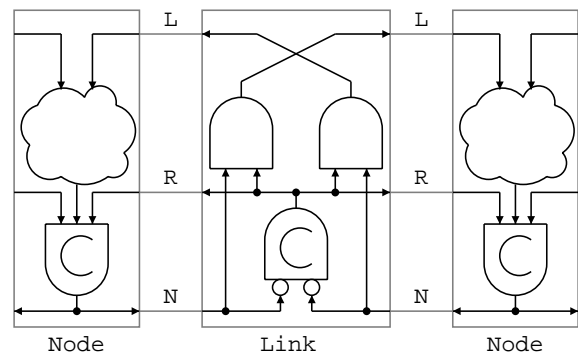
Figure 7: Counterflow network circuit
