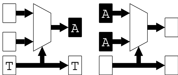
Figure 14: Anti-Token propagation
