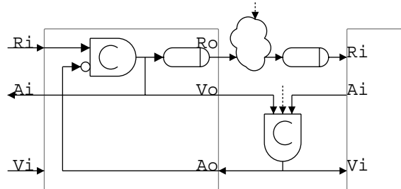
Figure 10: Validity signal connections
