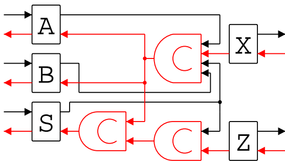
Figure 9: Guarding logic
