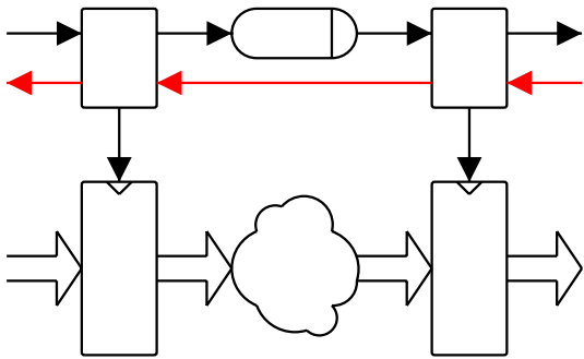
Figure 3: Asynchronous pipeline
