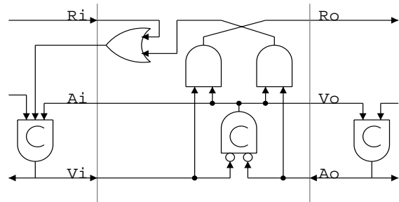
Figure 12: Adapted anti-token latch design
