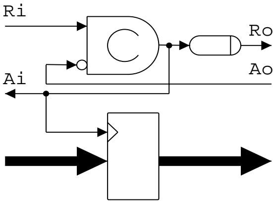
Figure 2: Example four phase latch
