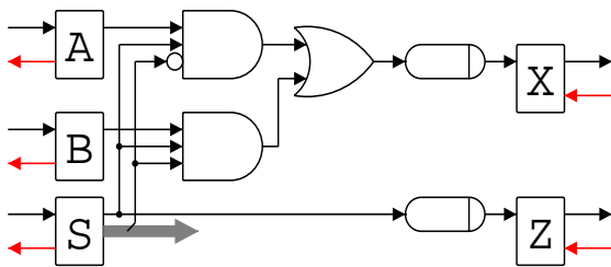
Figure 8: Early output request generation
