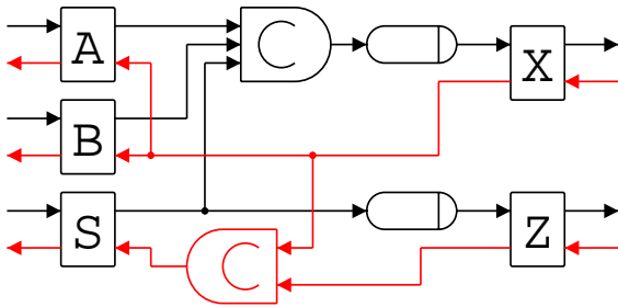
Figure 6: Standard request and acknowledge generation
